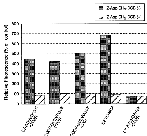
Fig. 4. Detection of caspase-3-like activity from HeLa-S3 cells treated with etoposide by using the synthetic fluorescent probes. All synthetic probes and DEVD-MCA were incubated for 2 h at 37°C with cell lysates of HeLa-S3 cells untreated (control) or treated with 20 \mu g/ml etoposide for 24 h. Z-Asp-CH 2 -DCB was added at 100 \mu M. Relative fluorescence is expressed as a percentage of control values. GDEVGVK and AYVHDAPVK are Gly-Asp-Glu-Val-Asp-Gly-Val-Lys and Ala-Tyr-Val-His-Asp-Ala-Pro-Val-Lys, respectively.
