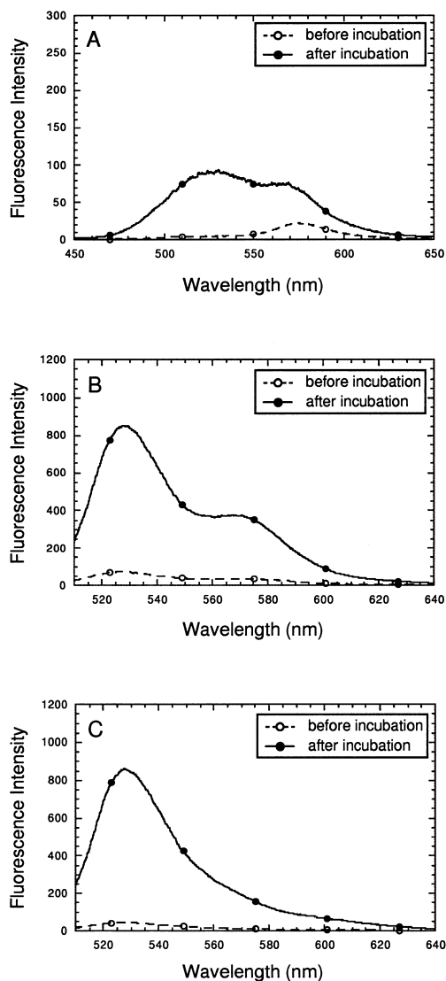
Fig. 2. Emission spectra of the synthetic fluorometric probes before (open circles) and after (closed circles) incubation with recombinant human caspase-3. A: LY-GDEVGDGVK-CTMR. B: CDCF-GDEVGDGVK-CTMR. C: CDCF-GDEVGDGVK-CXR. All synthetic probes (2 µM) were incubated with recombinant human caspase-3 (0.2 µg/ml) for 4 h at 37°C.
