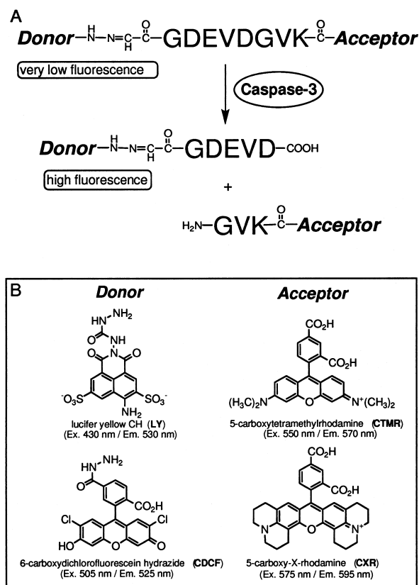
Fig. 1. A: Structure of the synthetic fluorometric probes and mechanism of detection of caspase-3. B: Structures of the fluorophores used as donors and the acceptors. GDEVGDGVK is Gly-Asp-Glu-Val-Asp-Gly-Val-Lys.
